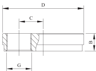
06P Cap with Eccentric Hole
